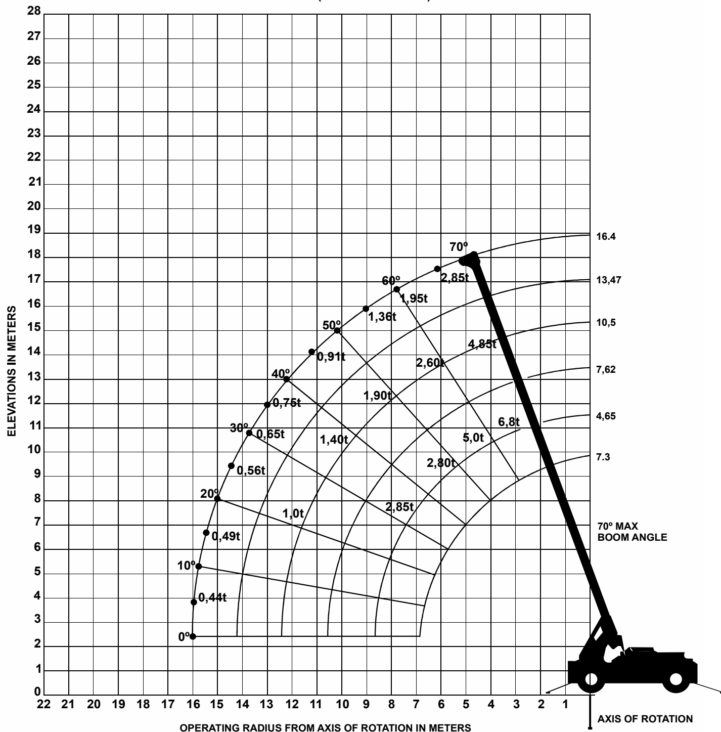
RANGE DIAGRAM (UNLADEN BOOM)
