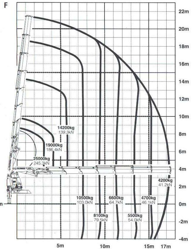
Madal/Palfinger PK100002 30t
